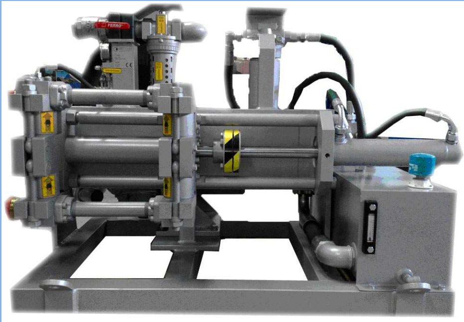
High pressure cement (laitance) pump
