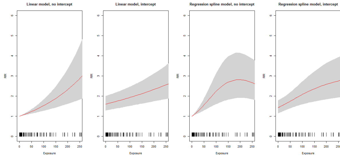
Figure 2. Meta-exposure-response relationships for cumulative asbestos fiber exposure and lung cancer based on data from 22 (cohort and case-control) studies based on modelling logRR on exposure using linear and spline models with and without intercepts. The fit of the different models is, using the Akaike Information Criterion from left to right 871.6, 137.7, 508.4, 114.7.
