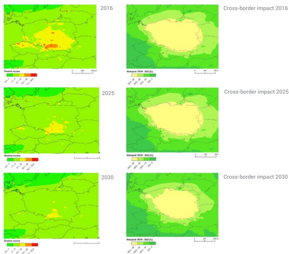
Figure 7. Spatial distribution of the average annual concentration of sulphur dioxide (left side) and spatial distribution of the impact index of the share of emissions from Poland for sulphur dioxide (right side) in 2016, 2025 and 2030.
