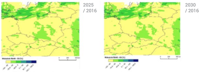
Figure 15. Relative change in AOT40 in 2025 (left panel) and 2030 (right panel) compared to 2016.
