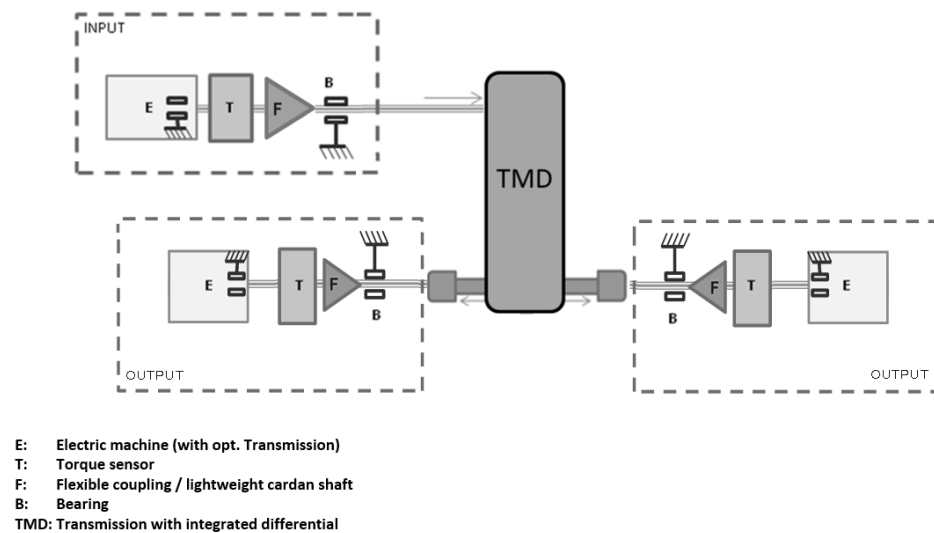
Test setup A for transmission with integrated differential
