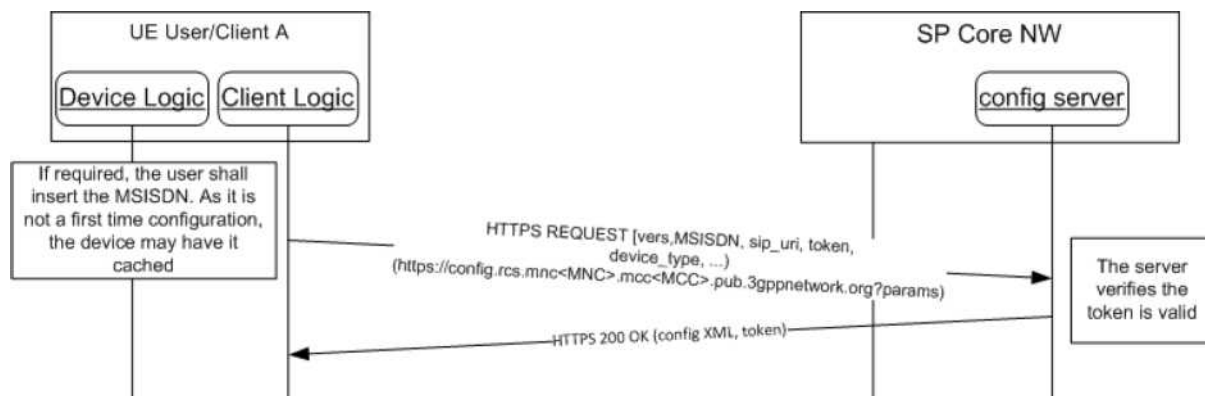
Figure 14: HTTP configuration for non-cellular devices: Subsequent attempts
