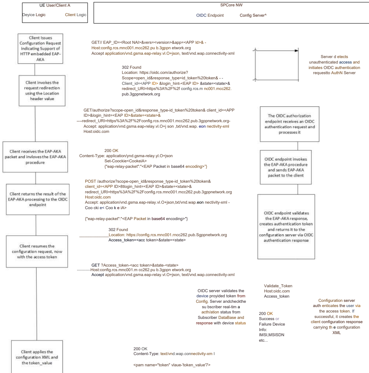
Figure 10: Authentication Flow using HTTP embedded EAP-AKA
